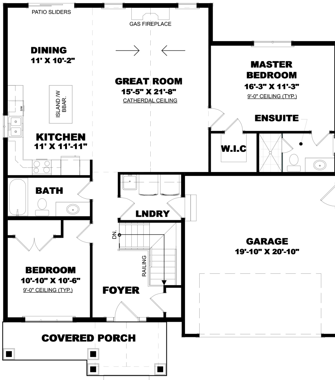
MAIN FLOOR
